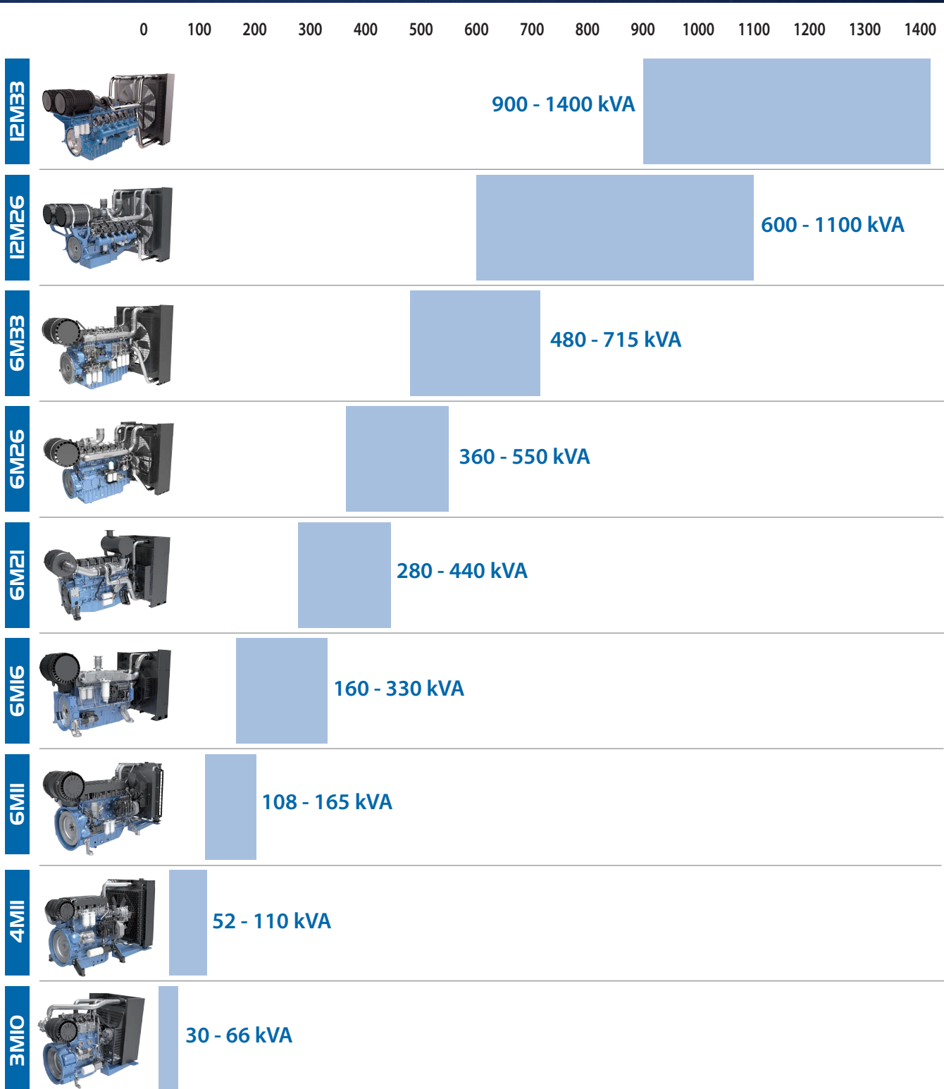
Typical Genset Output (kVA) @ 50 Hz
